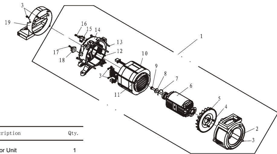
(2)Motor Assembly
