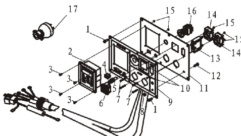
(9)Control Panel
