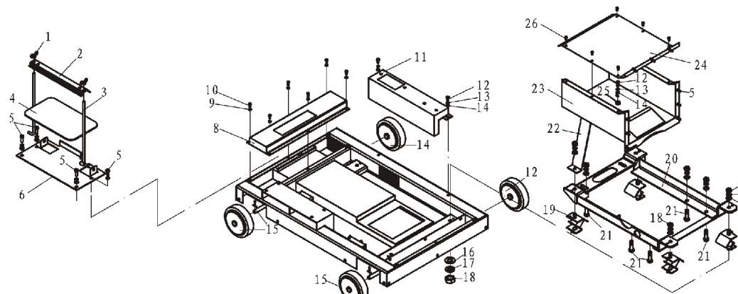
(3)Chassis Assembly
